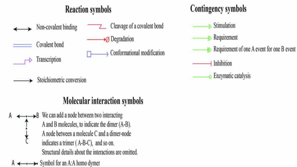
Figure 1: Molecular Interaction Map (MIM) (above), including most of the G0-G1 transition signaling-network, in Colorectal Cancer . The cartouches (like in hieroglyphics), contain the signaling-proteins of the network. The MIM syntax (panel B) is according to [Kohn, K.W. et al., (2006). Mol Syst Biol 2:51]. Numbers near the interaction lines refer to an Annotation list of interactions and a Glossary(supplementary material of [Tortolina, L. et al., (2015). Oncotarget 6(7) 5041-58]) continuously updated. Grid cordينات (numbers at the left and letters on the top of the MIM) help to locate molecular species and interactions present in the MIM.
